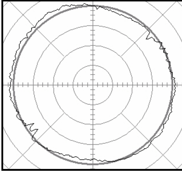
HORIZONTAL PROFILE
